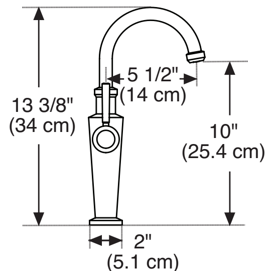
Dimensional Drawing
